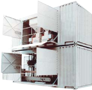
Mobile bagging units (containerized)
